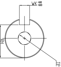
SHAFT END DETAIL
