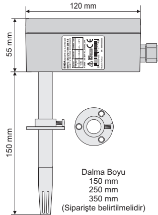
EHTC-DC-xV-x50-xx-xx KANAL MONTAJLI TİP
