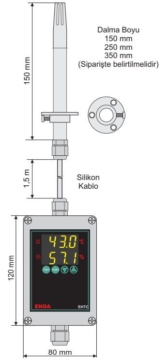
EHTC-CB-xV-x50-xx-xx KABLOLU TİP
